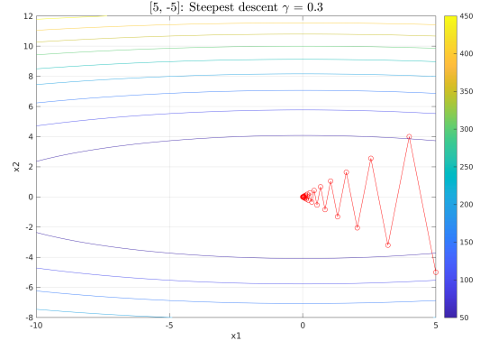
\gamma_k = 0.3
