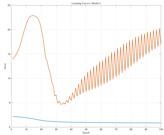
(β') Learning curves — Model 4
