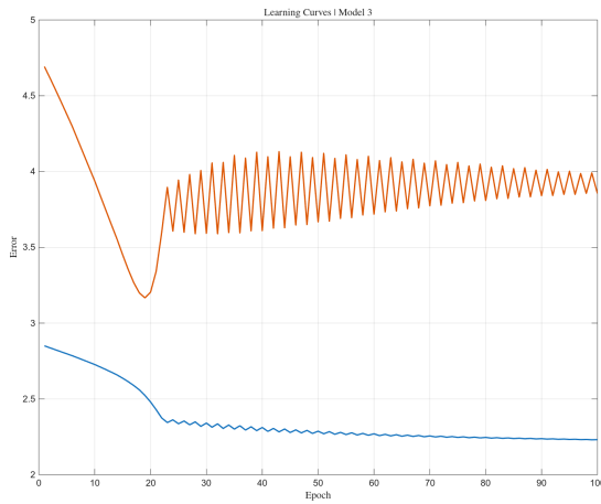
(α') Learning curves — Model 3
